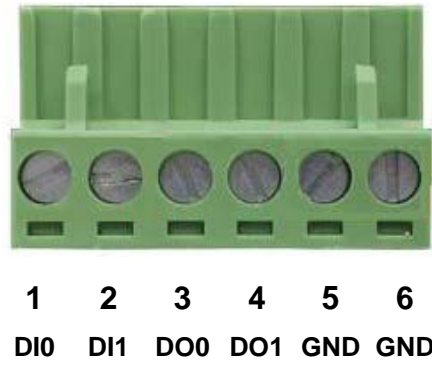
Figure 2-15: 6-pin Terminal Block for DI and DO Wiring Input
