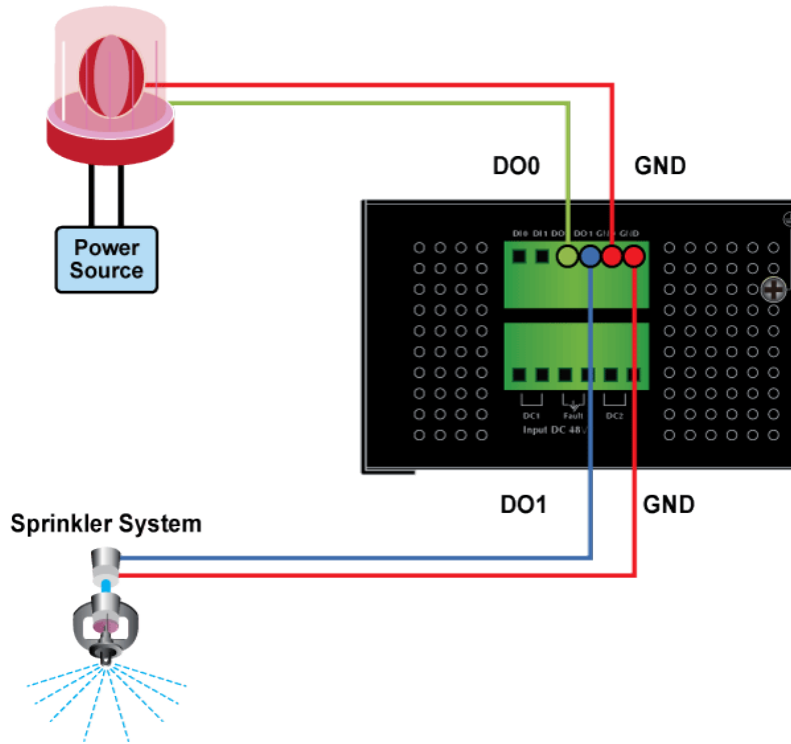
Figure 2-17: Wiring DO0 and DO1 to Open Detector
