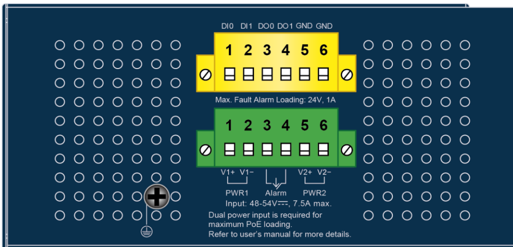
Figure 2-1-4c: Industrial Managed Switch Upper Panel.
