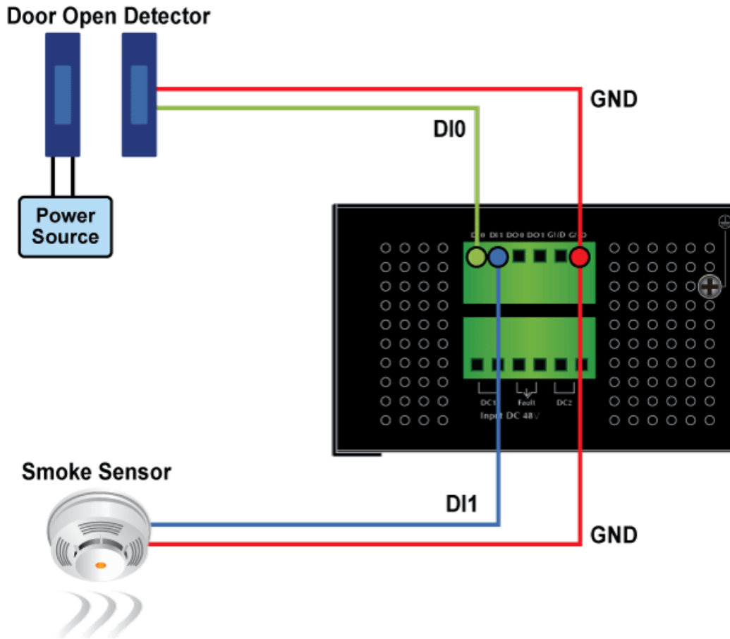
Figure 2-1-7c Wiring DI0 and DI1 to Open Detector
