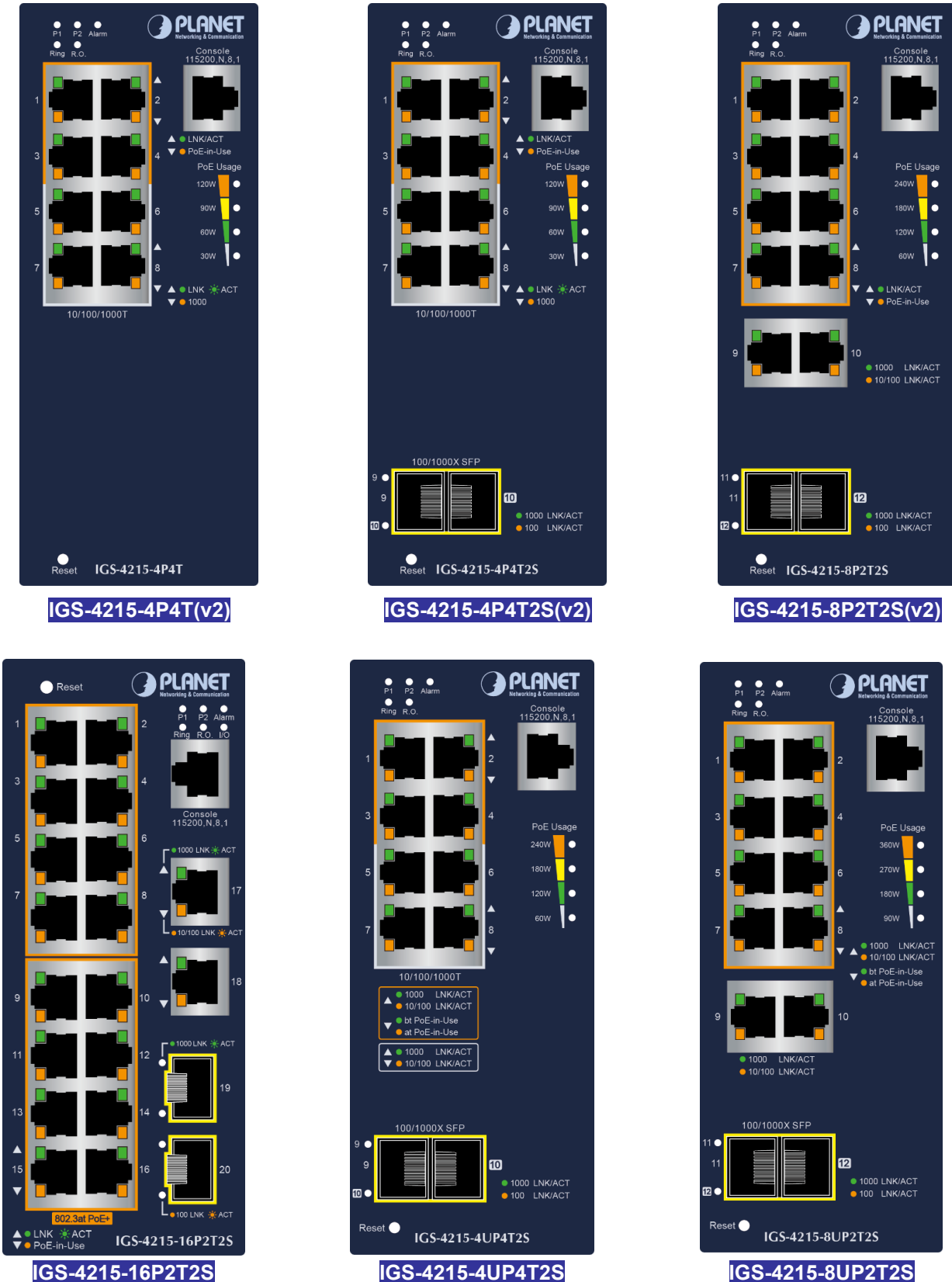
Figure 2-1-2a: IGS-4215 PoE series' Front Panels
