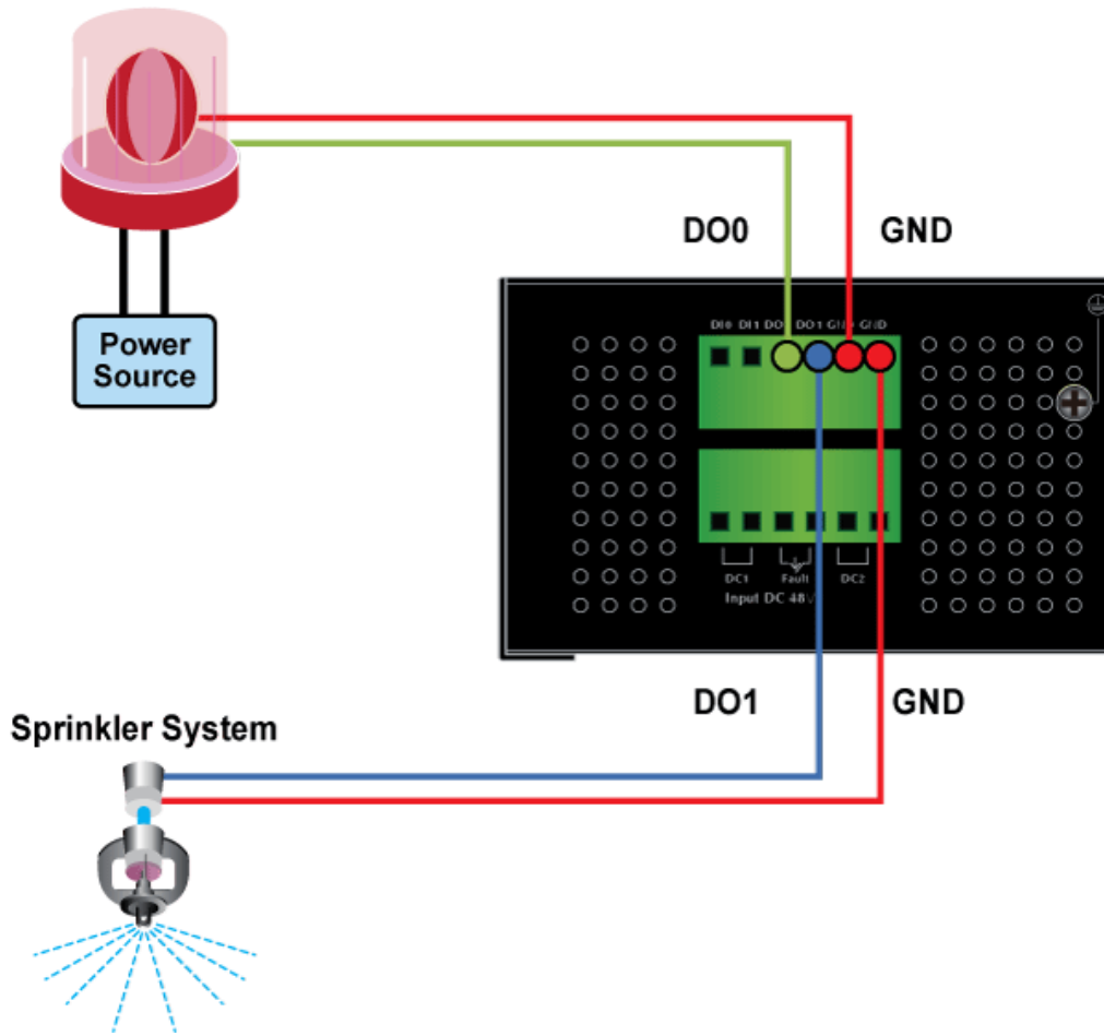
Figure 2-1-7d Wiring DO0 and DO1 to Open Detector
