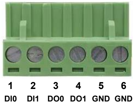
Figure 2-1-7b 6-pin Terminal Block for DI and DO Wiring Input
