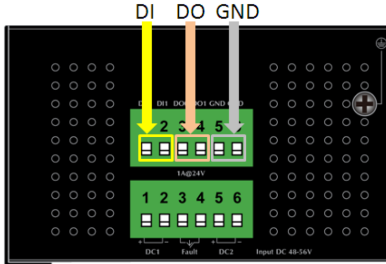
Figure 2-1-7a Wiring the Redundant Power Inputs
